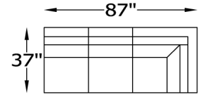
135315L or R ARMLESS SOFA WITH RETURN SHOWN AS A RIGHT
